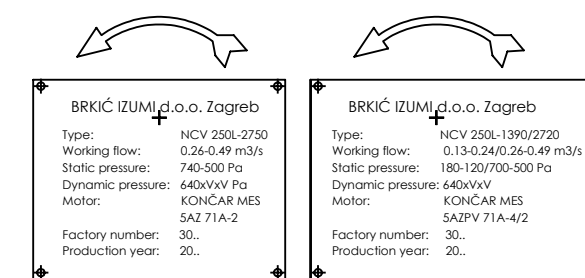
Type 3 Nameplate Type 4 Nameplate
