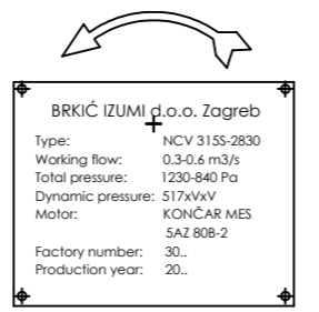
Type 7 Nameplate
